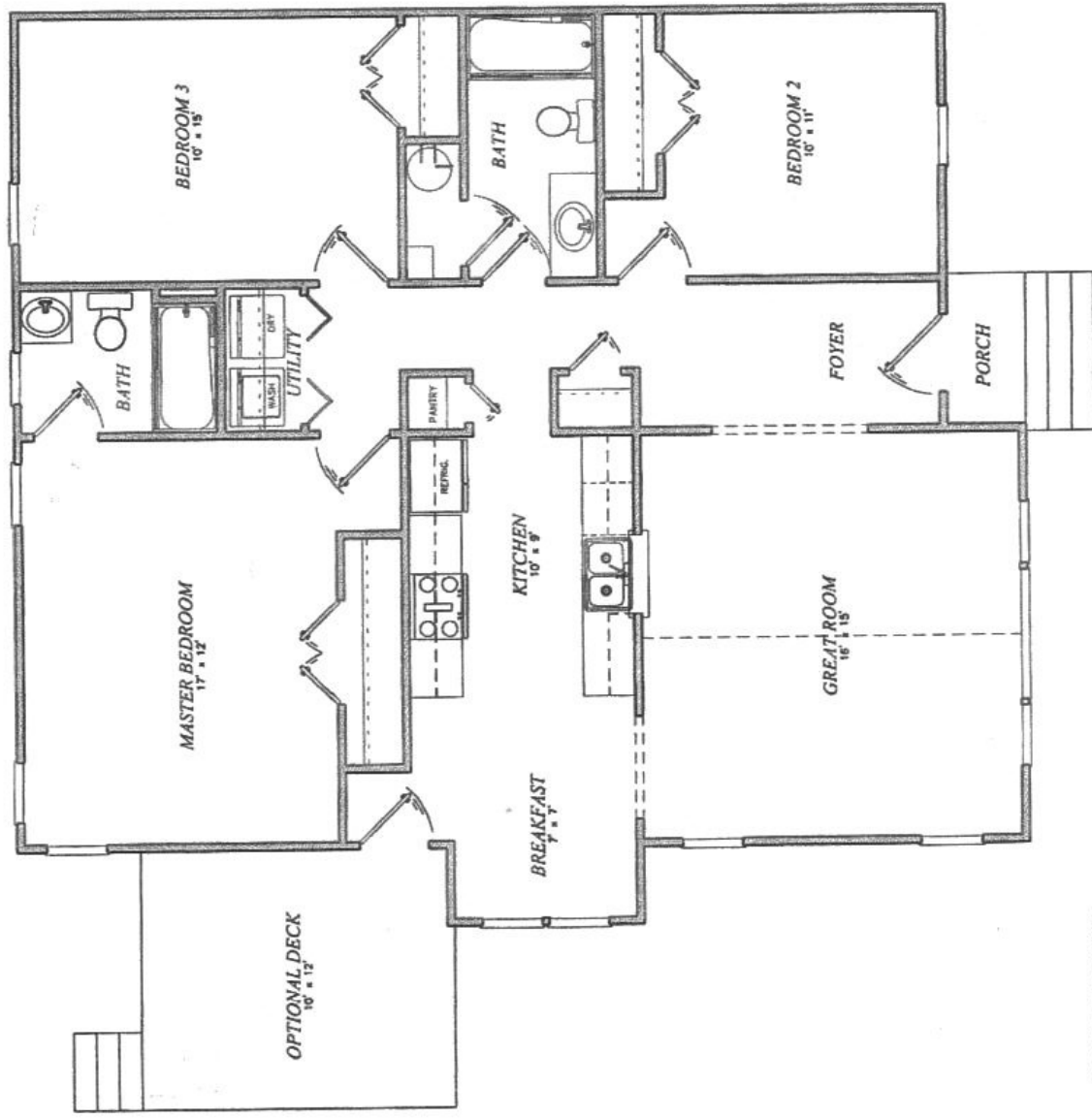
FLOOR PLAN
